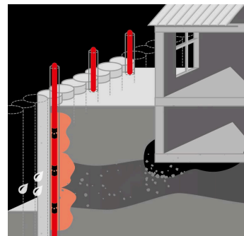
Consolidation and sealing of a bored pile wall
